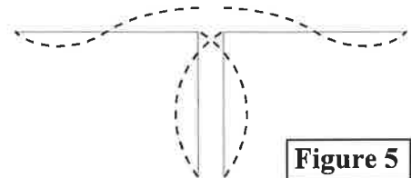
Current Distribution 18MHz
