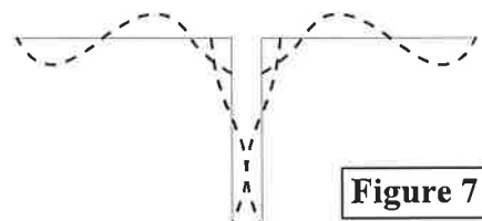
Current Distribution 24MHz
